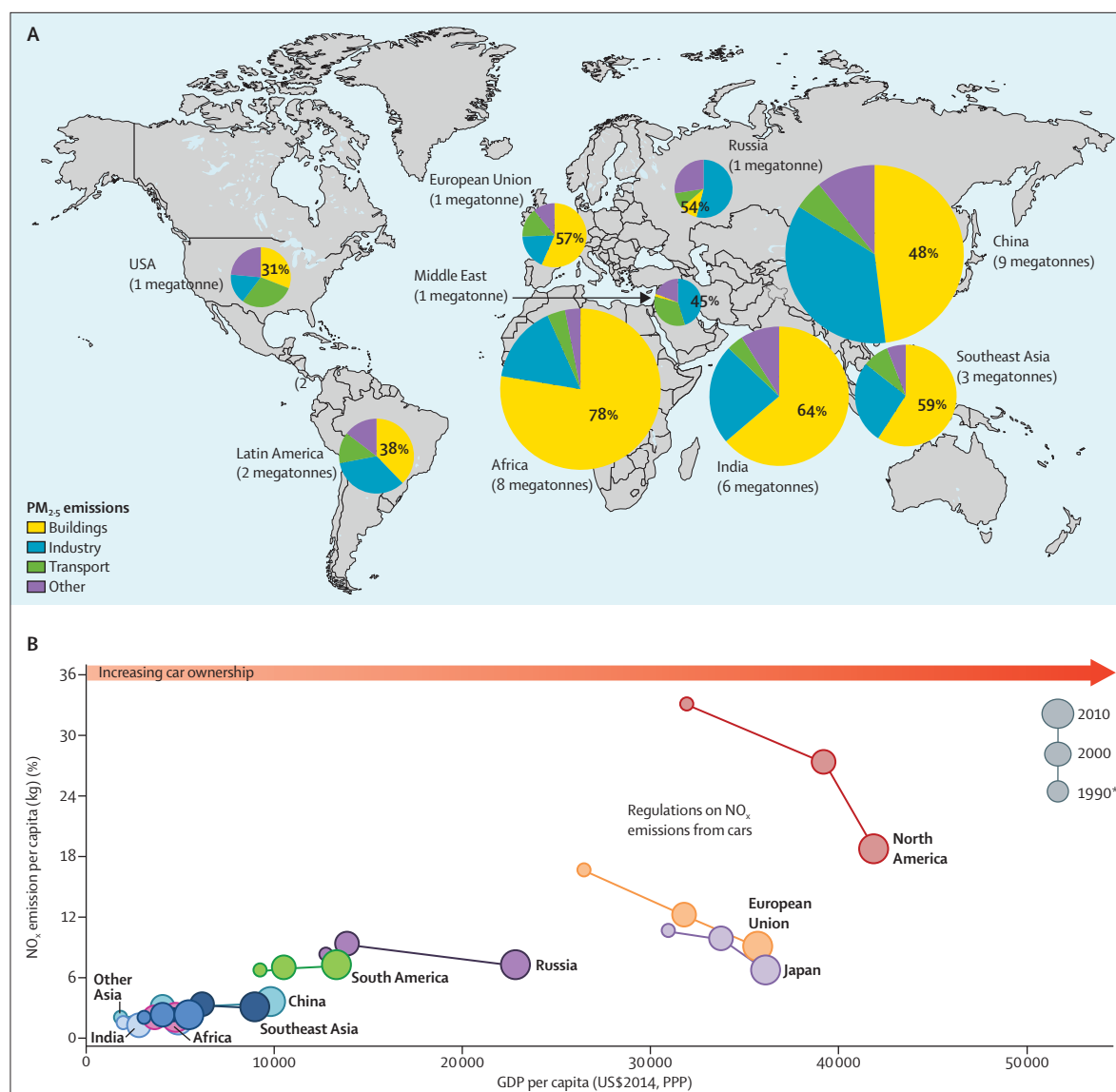
Figure 23: Sources and trends in particulate pollution
